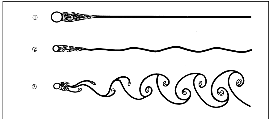
Vortex pattern downstream of a cylinder in a range of very low Reynolds' numbers according to Homann.
